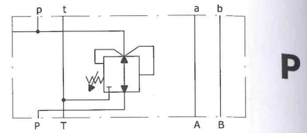
O-Ring side
